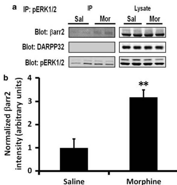
Figure 3 \beta -Arrestin2 and pERK form a complex on morphine stimulation. (a) Immobilized pERK antibody agarose beads were mixed with striatal lysates from saline (Sal, n = 6 ) or morphine (Mor, n = 6 ) (20 mg/kg, s.c.), injected into C57Bl/6J WT mice, and subjected to western blot as described in the 'Materials and methods' section. Membranes were probed with antibodies to \beta arr2, DARPP-32, and pERK. The left-side panel represents the immunoprecipitated protein and right panel the total lysates. (b) \beta arr2 band intensity was quantified using ImageJ and normalized to pERK (loading control) band intensity. ** p < 0.01 , compare saline with morphine.
